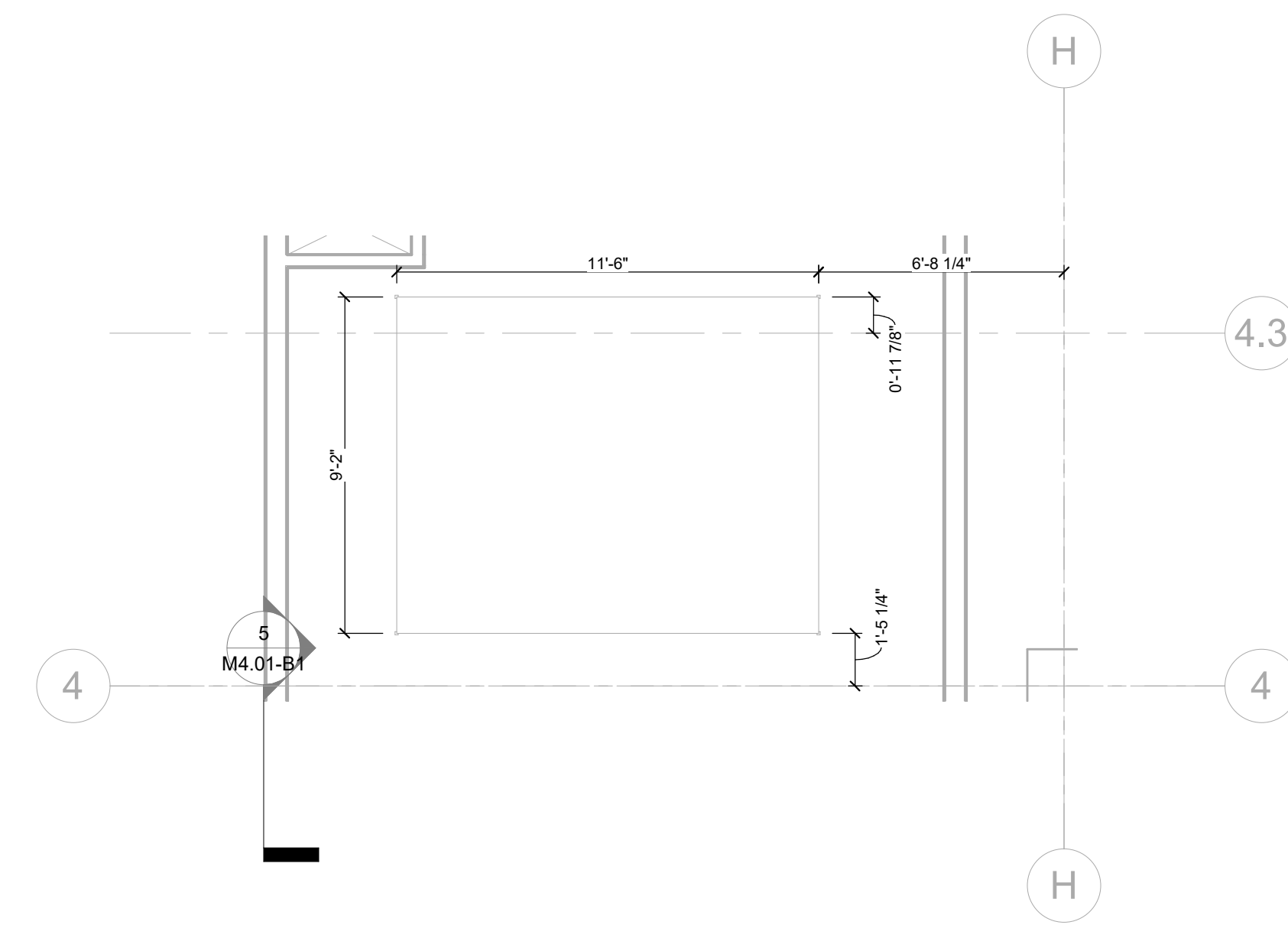
7 LEVEL 7 HVAC PRINT - B1 - EQUIPMENT PAD 1/4" = 1'-0"
