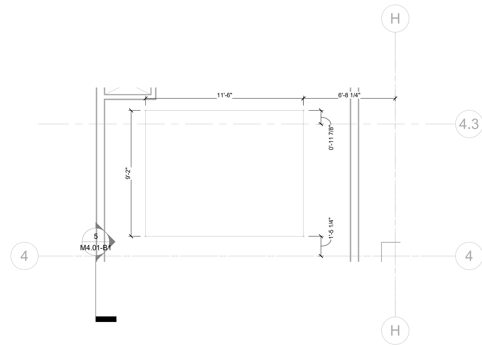
8 LEVEL 8 HVAC PRINT - B1 - EQUIPMENT PAD 1/4" = 1'-0"
