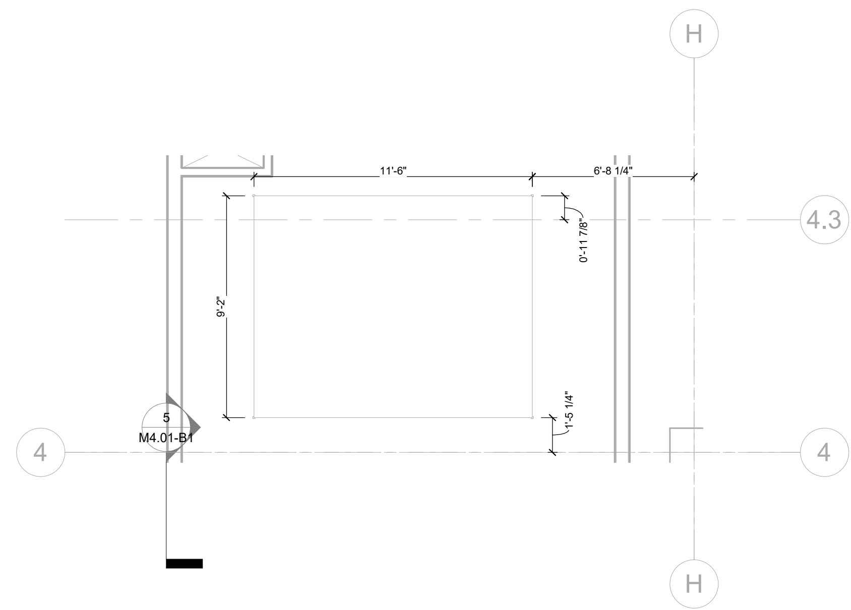
6 LEVEL 6 HVAC PRINT - B1 - EQUIPMENT PAD 1/4" = 1'-0"
