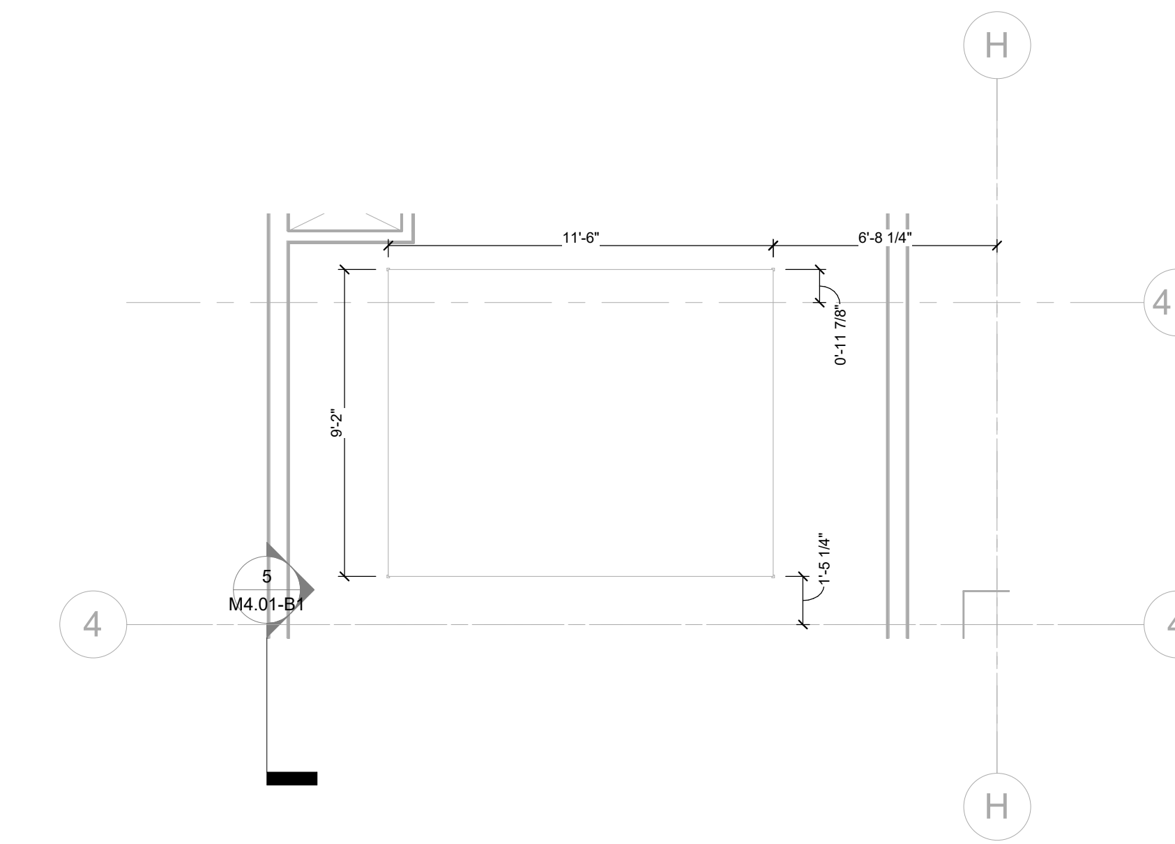
10 LEVEL 10 HVAC PRINT - B1 - EQUIPMENT PAD 1/4" = 1'-0"
