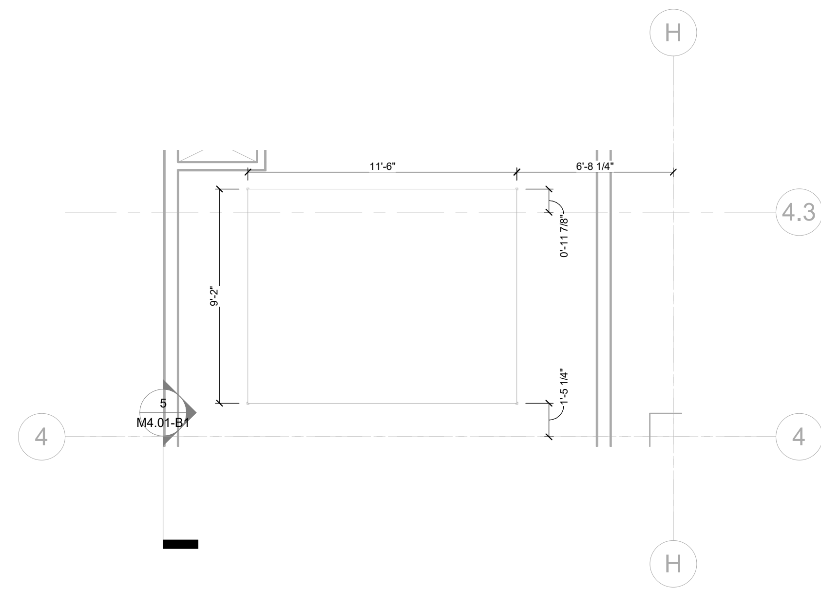
5 LEVEL 5 HVAC PRINT - B1 - EQUIPMENT PAD 1/4" = 1'-0"
