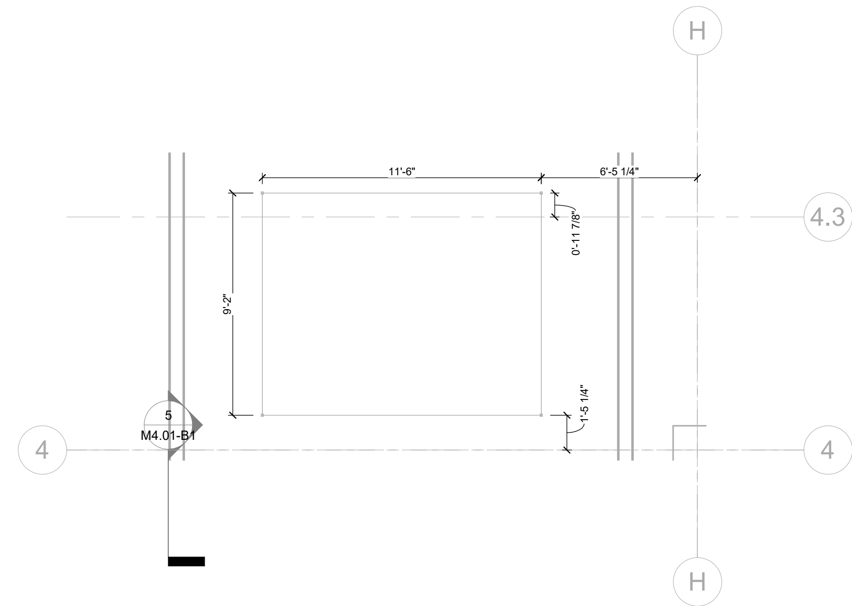
2 Level 2 HVAC PRINT - B1 - EQUIPMENT PAD 1/4" = 1'-0"
