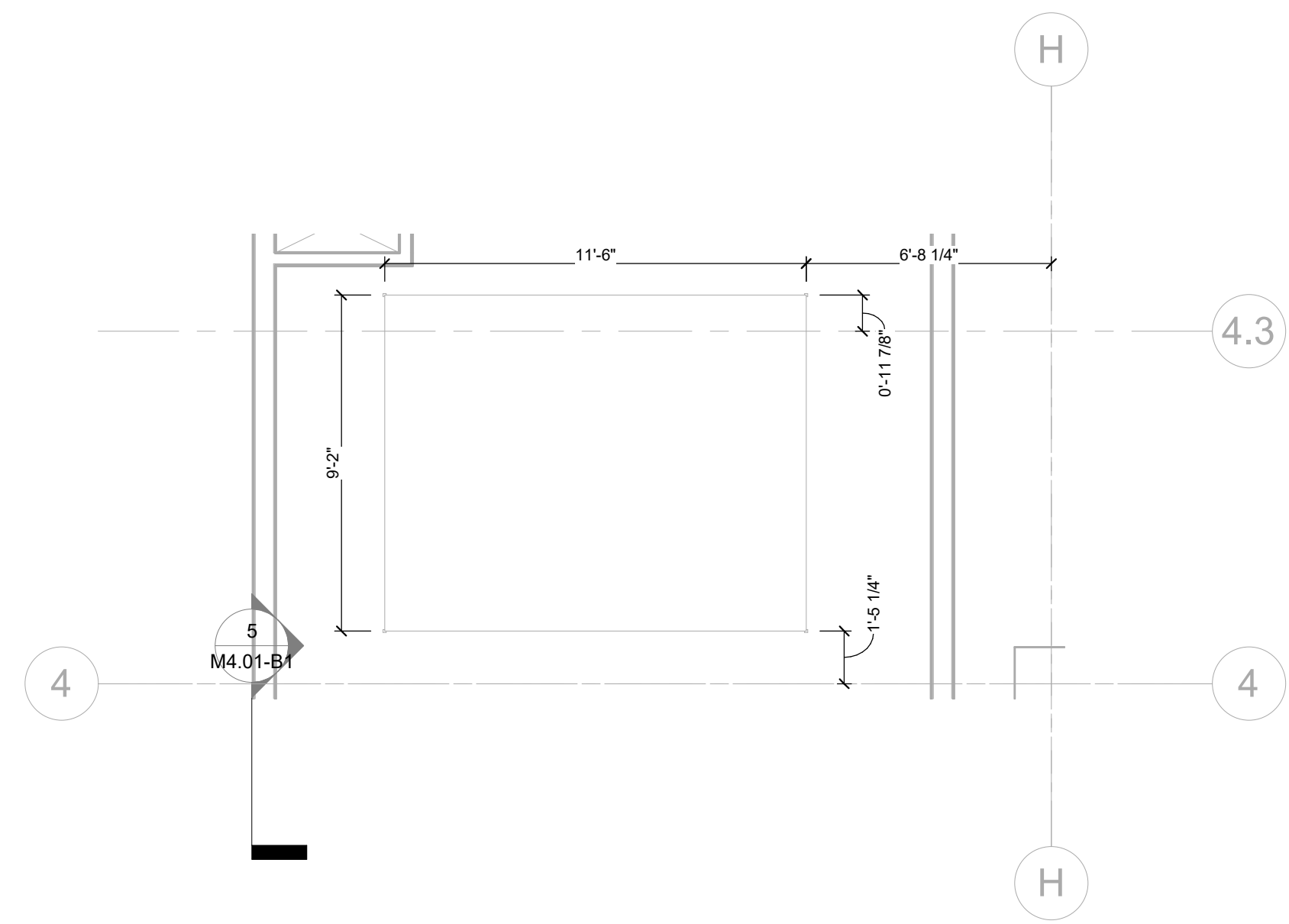
9 LEVEL 9 HVAC PRINT - B1 - EQUIPMENT PAD 1/4" = 1'-0"
