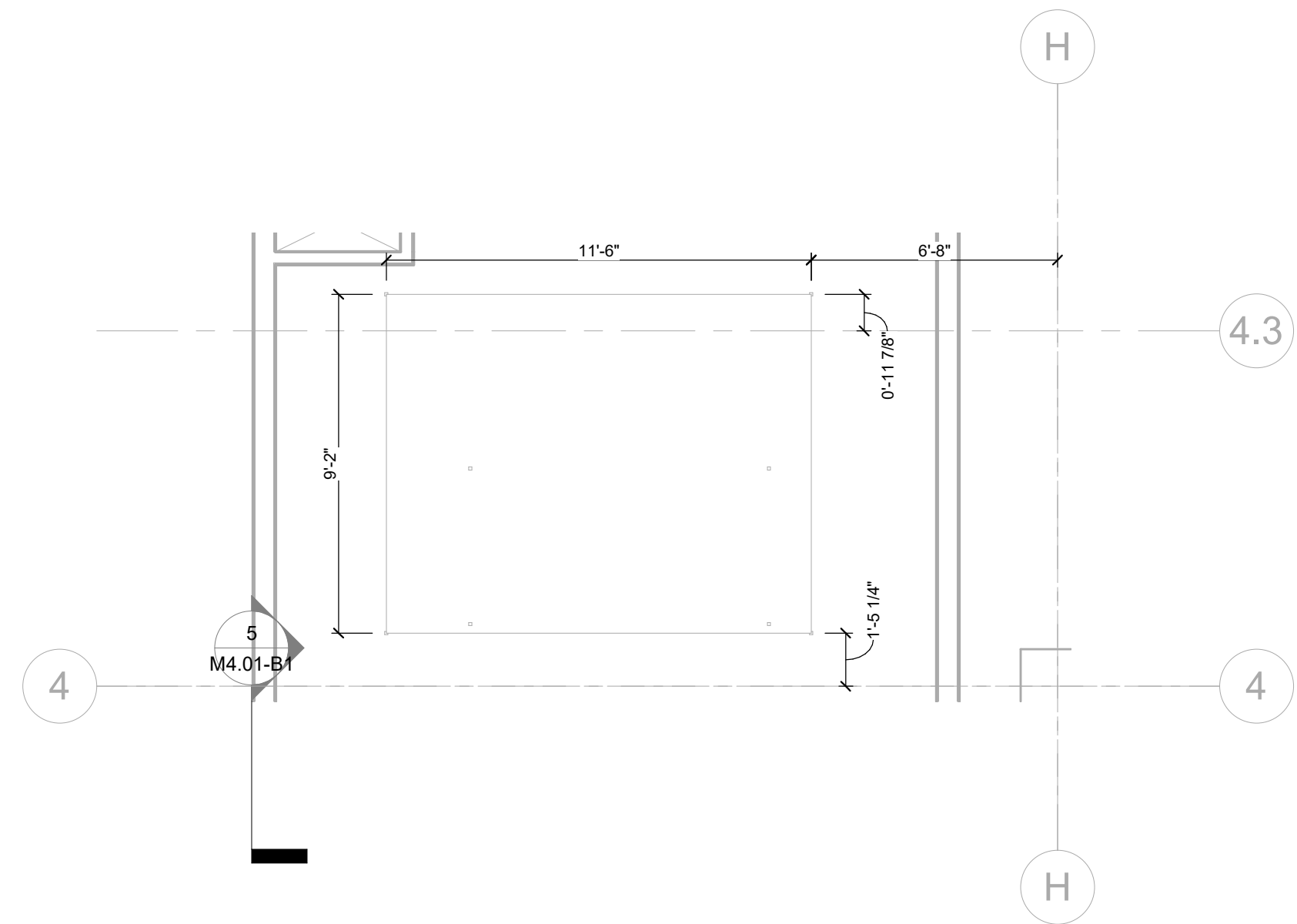
4 LEVEL 4 HVAC PRINT - B1 - EQUIPMENT PAD 1/4" = 1'-0"
