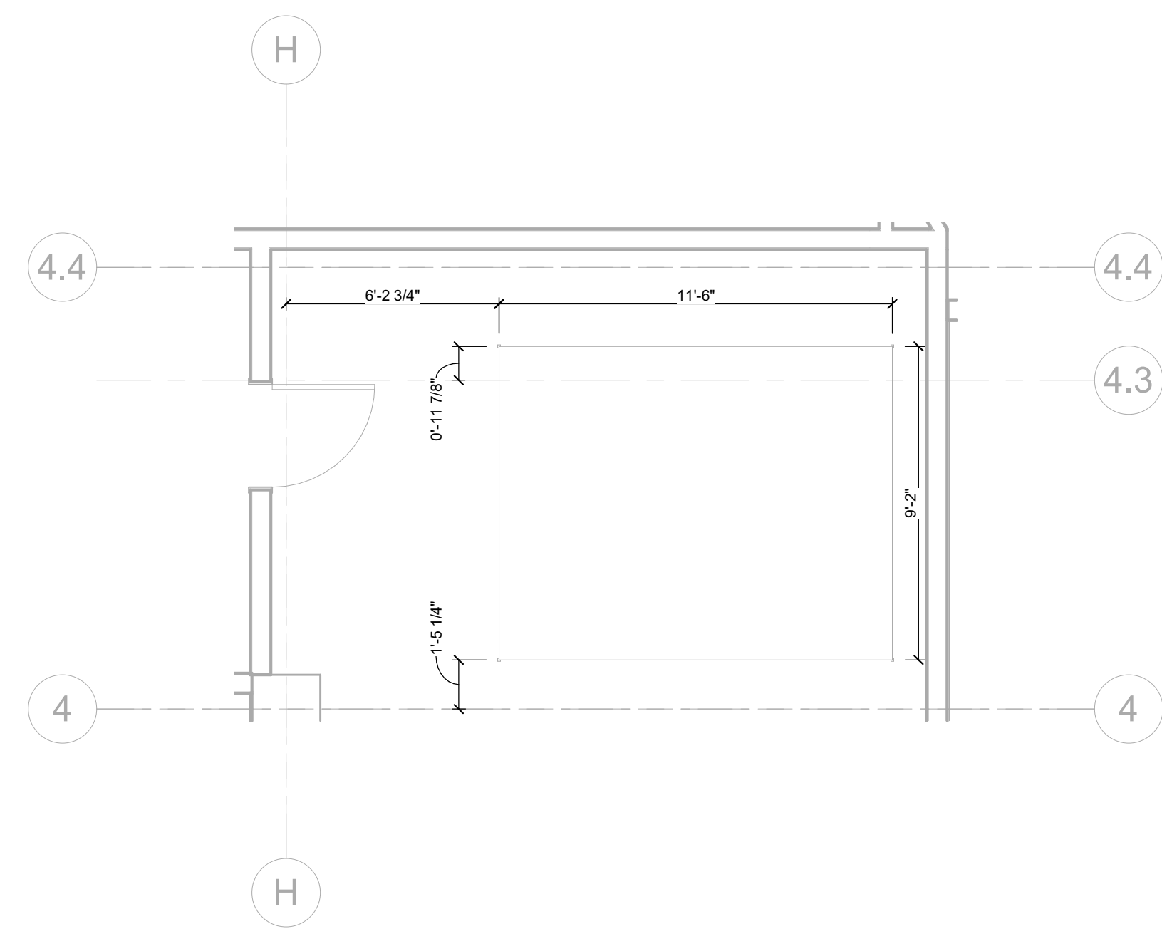
1 Level 1 HVAC PRINT - B1 - EQUIPMENT PAD 1/4" = 1'-0"
