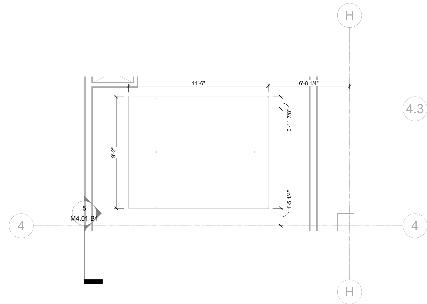
3 LEVEL 3 HVAC PRINT - B1 - EQUIPMENT PAD 1/4" = 1'-0"
