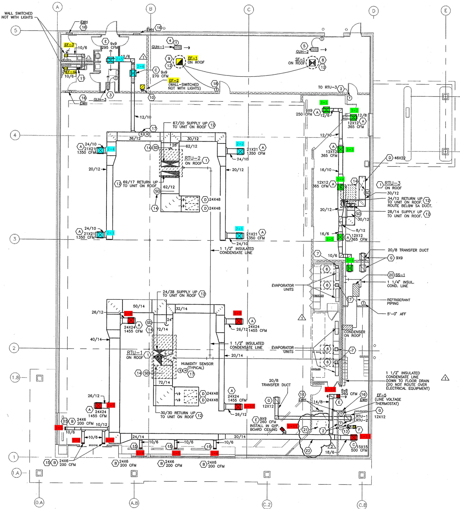
FLOOR PLAN - MECHANICAL
