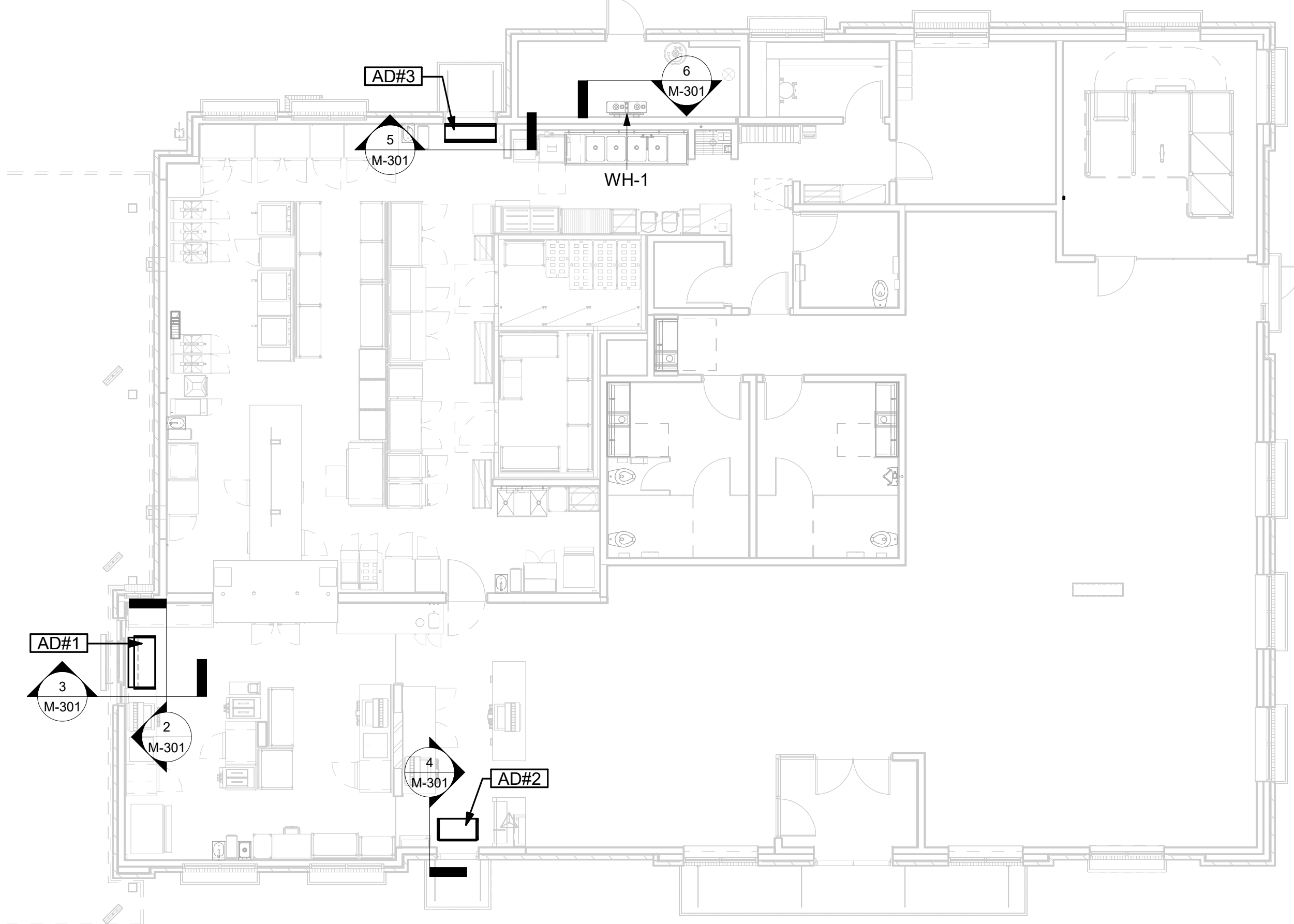
1 VARIOUS SECTIONS 1/8" = 1'-0"
