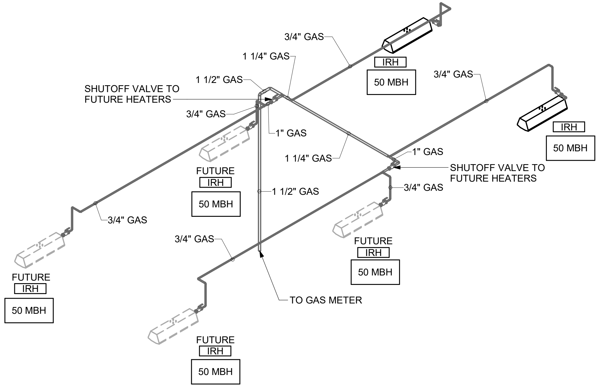
2 GAS PIPING ISOMETRIC - ORDER CANOPY
