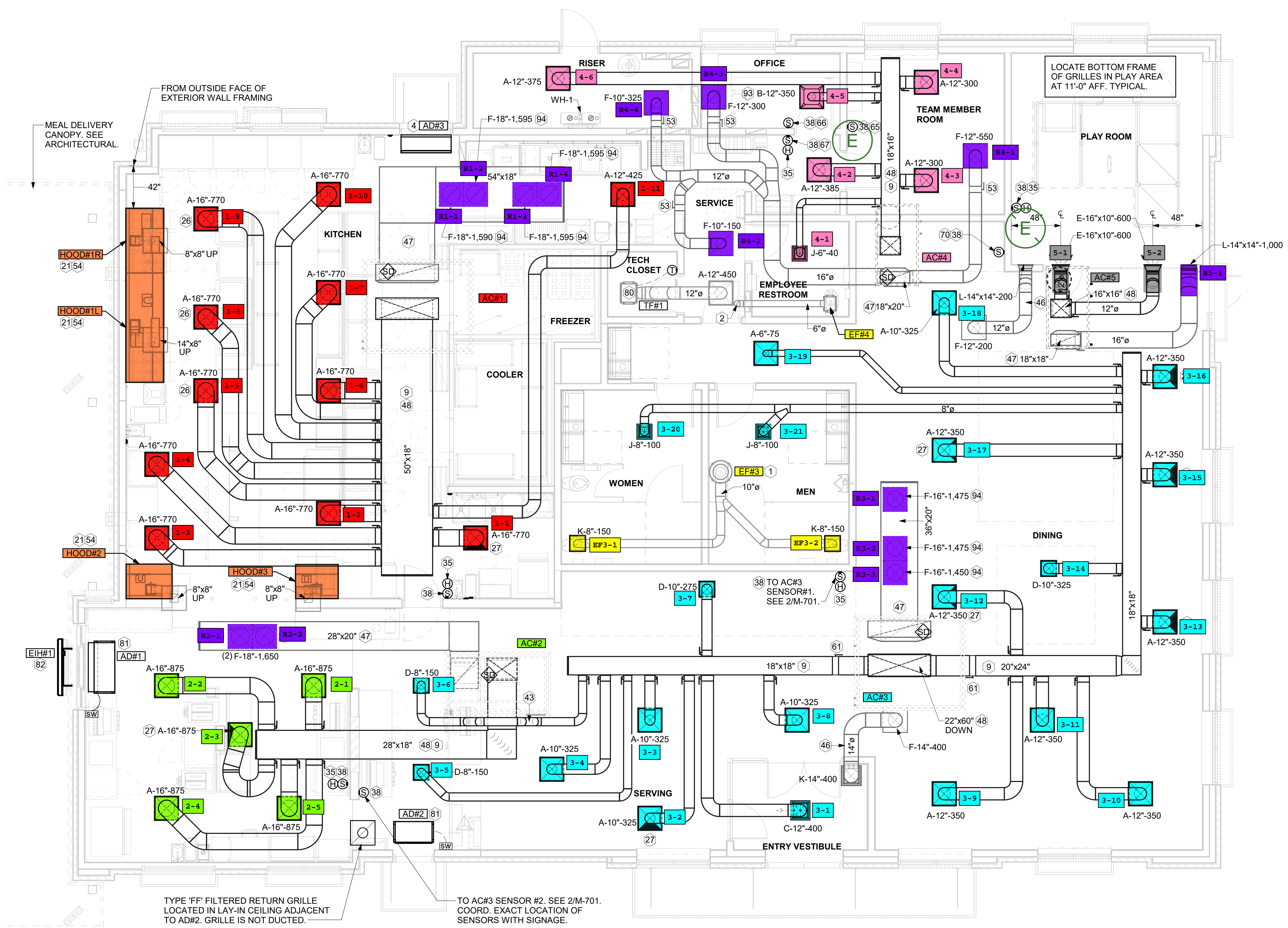
1 EQUIPMENT AND DUCTWORK PLAN 1/4" = 1'-0"
