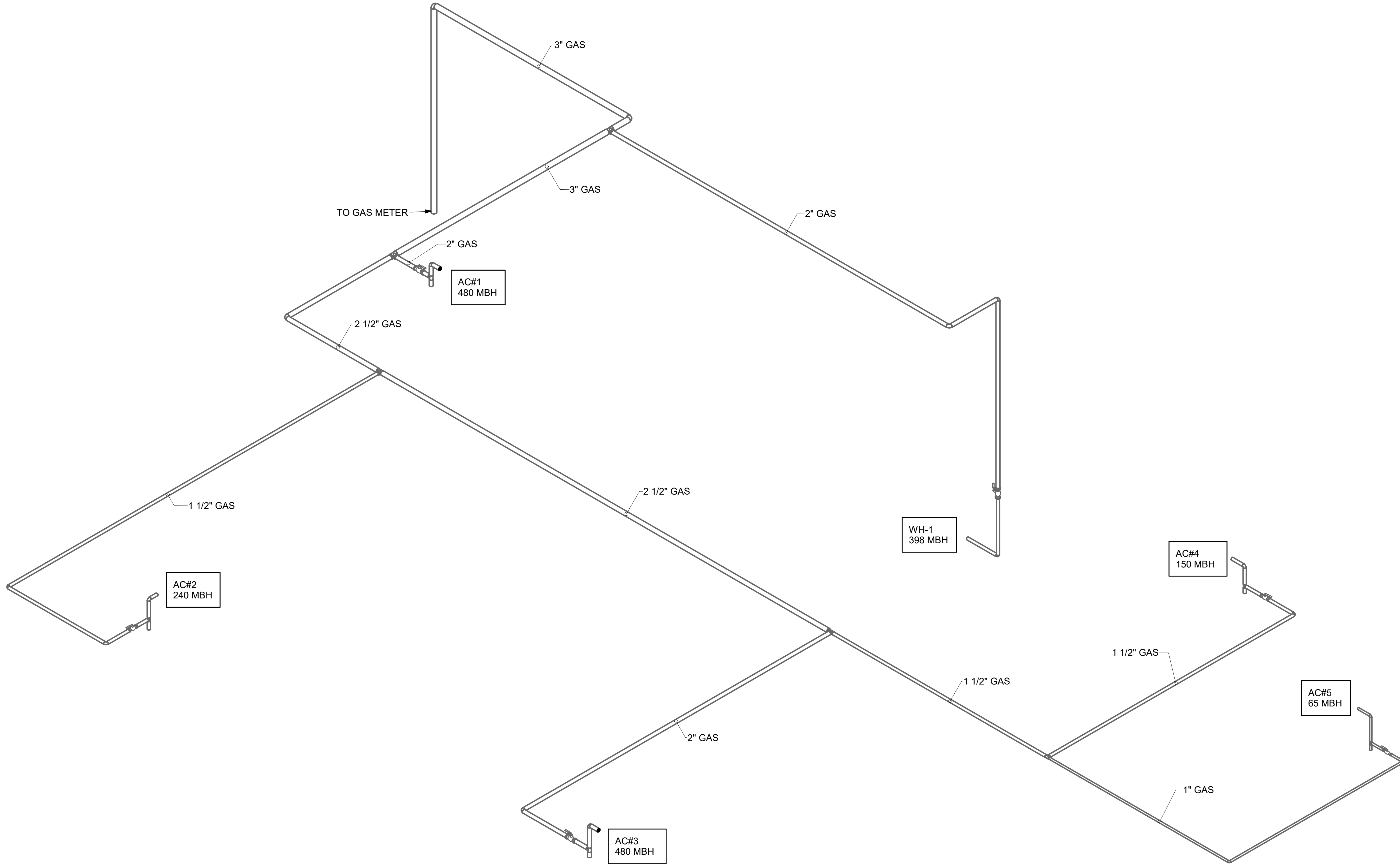
1 GAS PIPING ISOMETRIC - RTUS AND WATER HEATER
