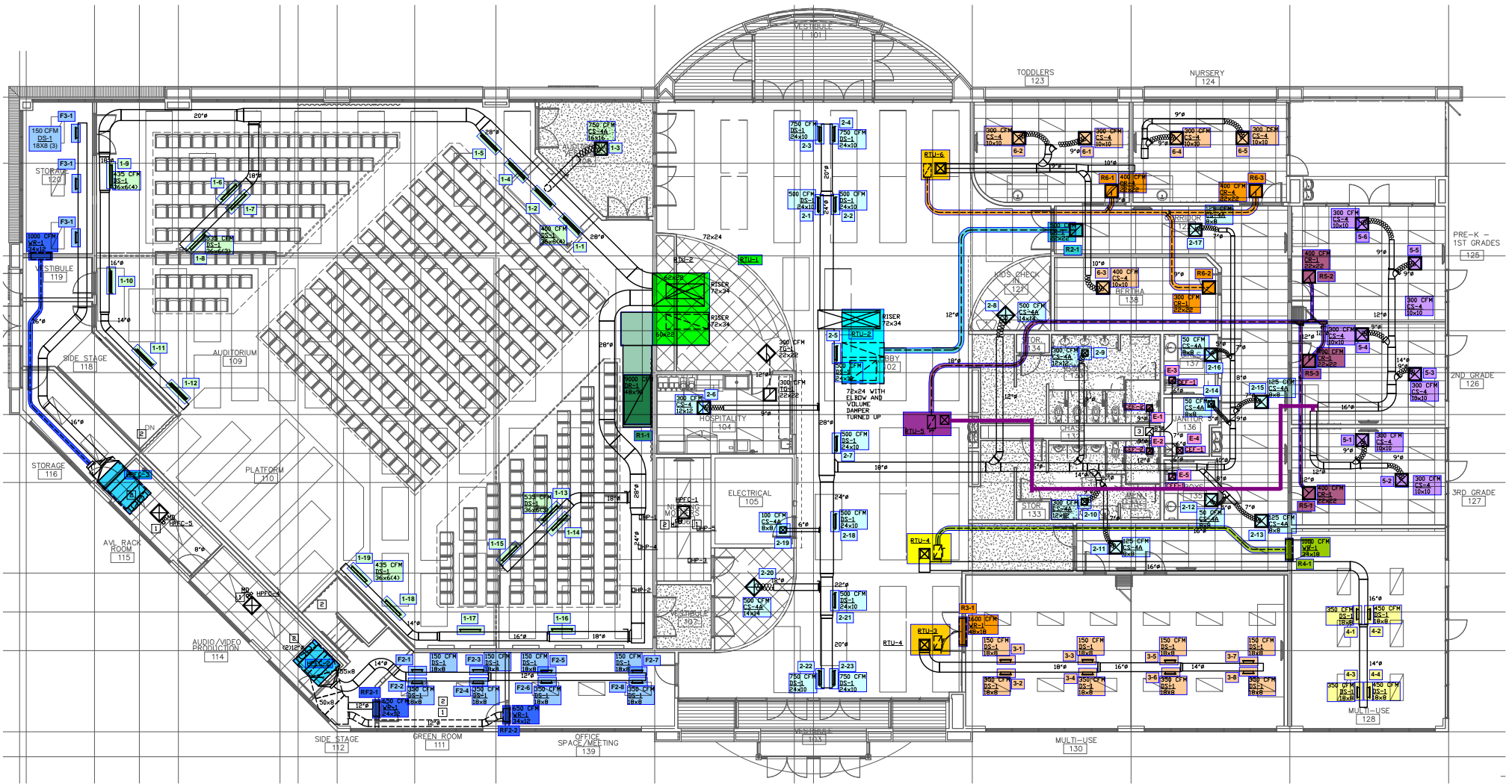
MECHANICAL FLOOR PLAN
