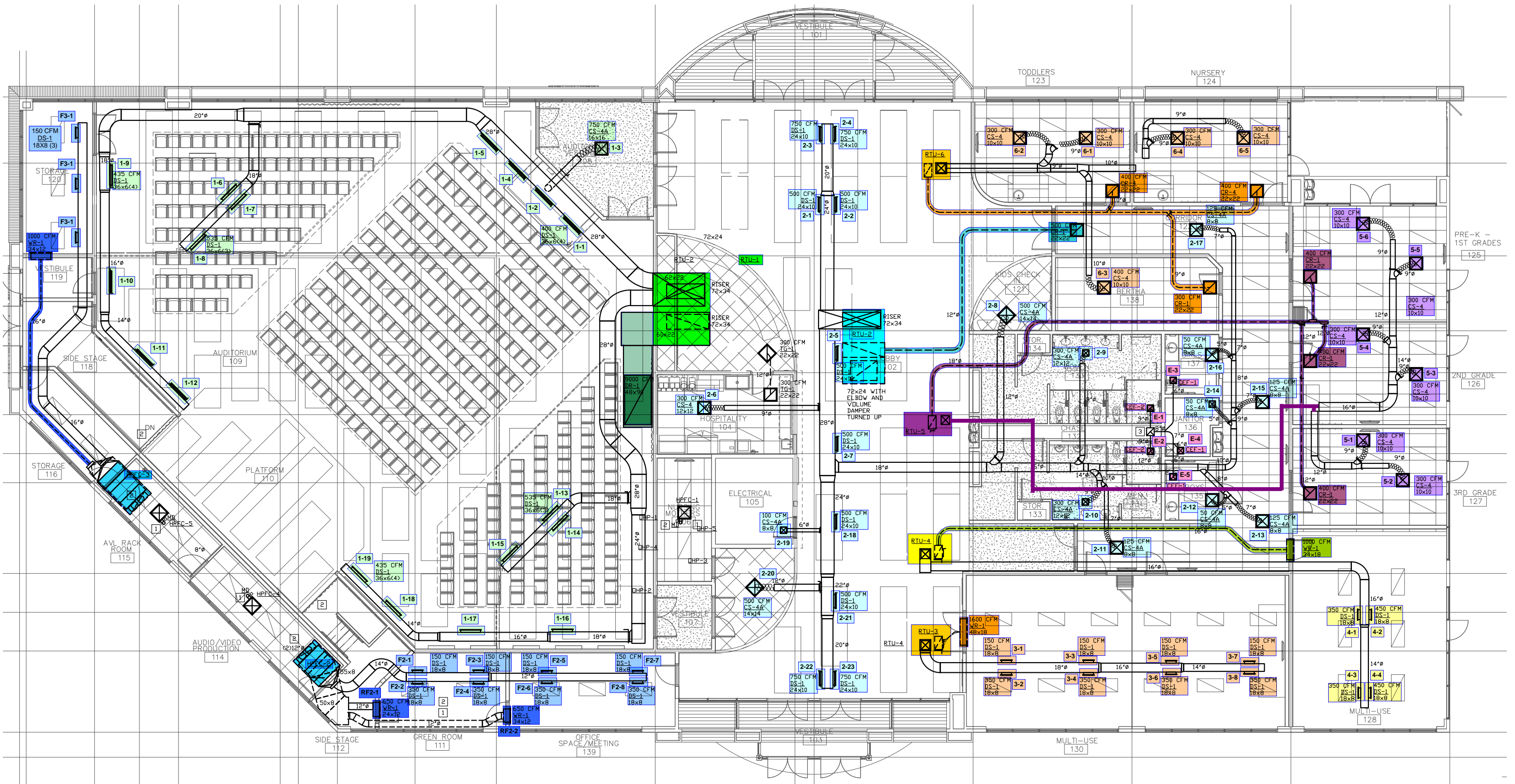
MECHANICAL FLOOR PLAN
