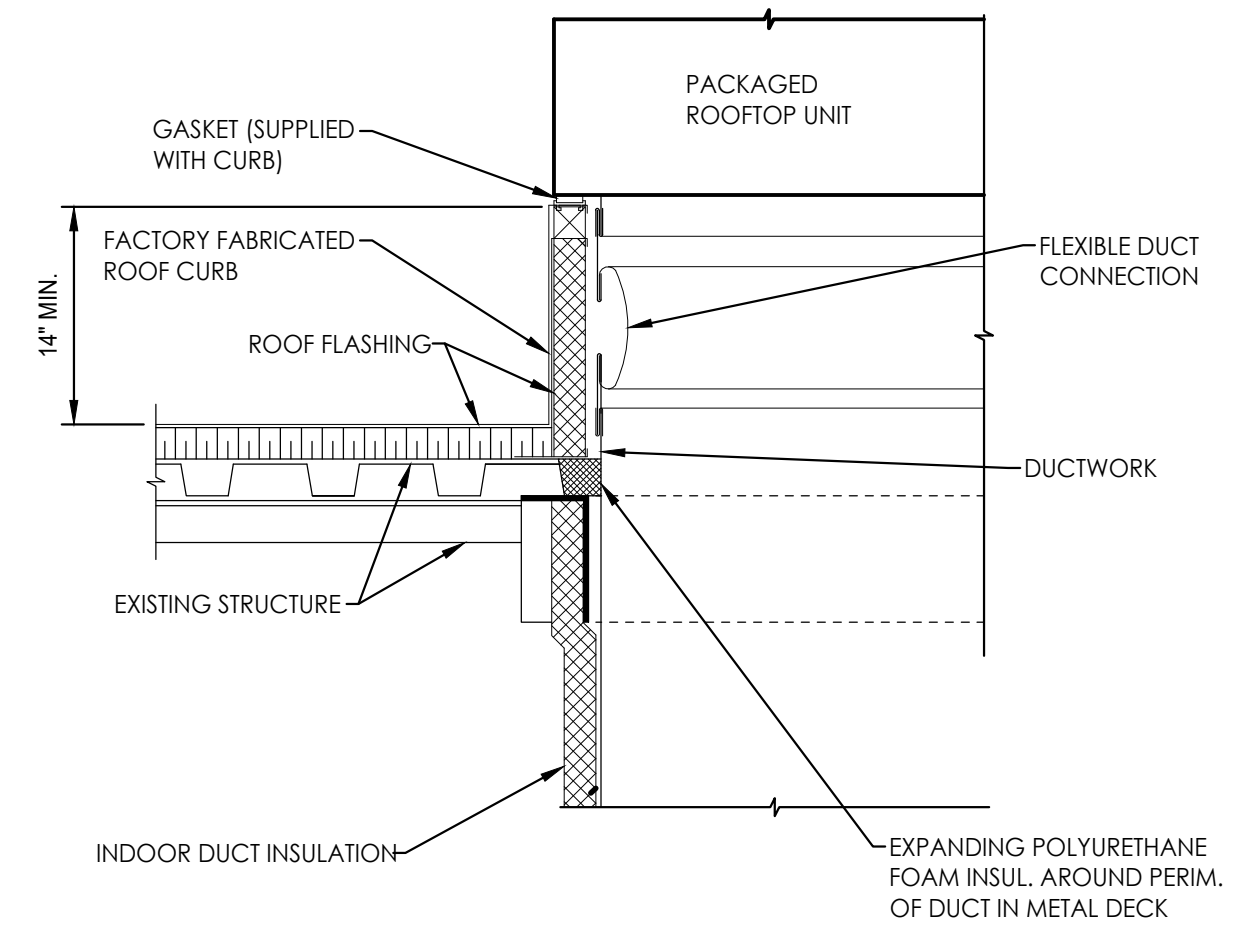
3 PACKAGED ROOFTOP UNIT DETAIL N.T.S.
