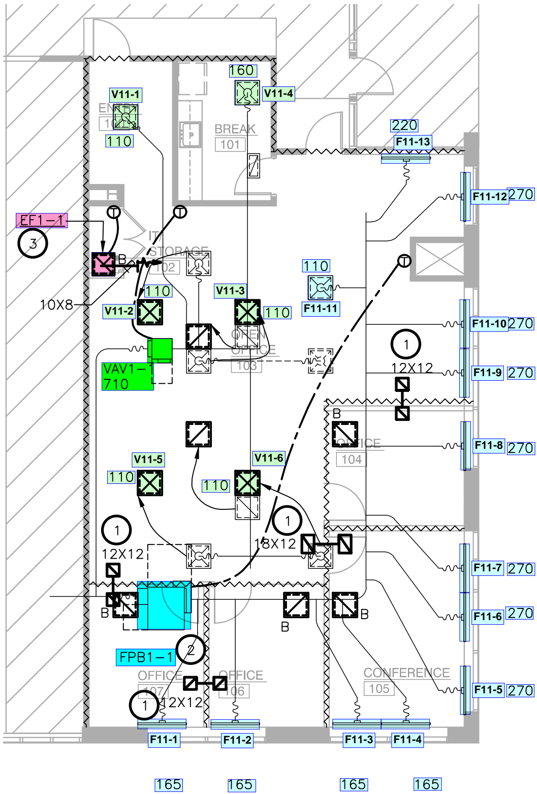
① LEVEL 01 MECHANICAL PLAN
