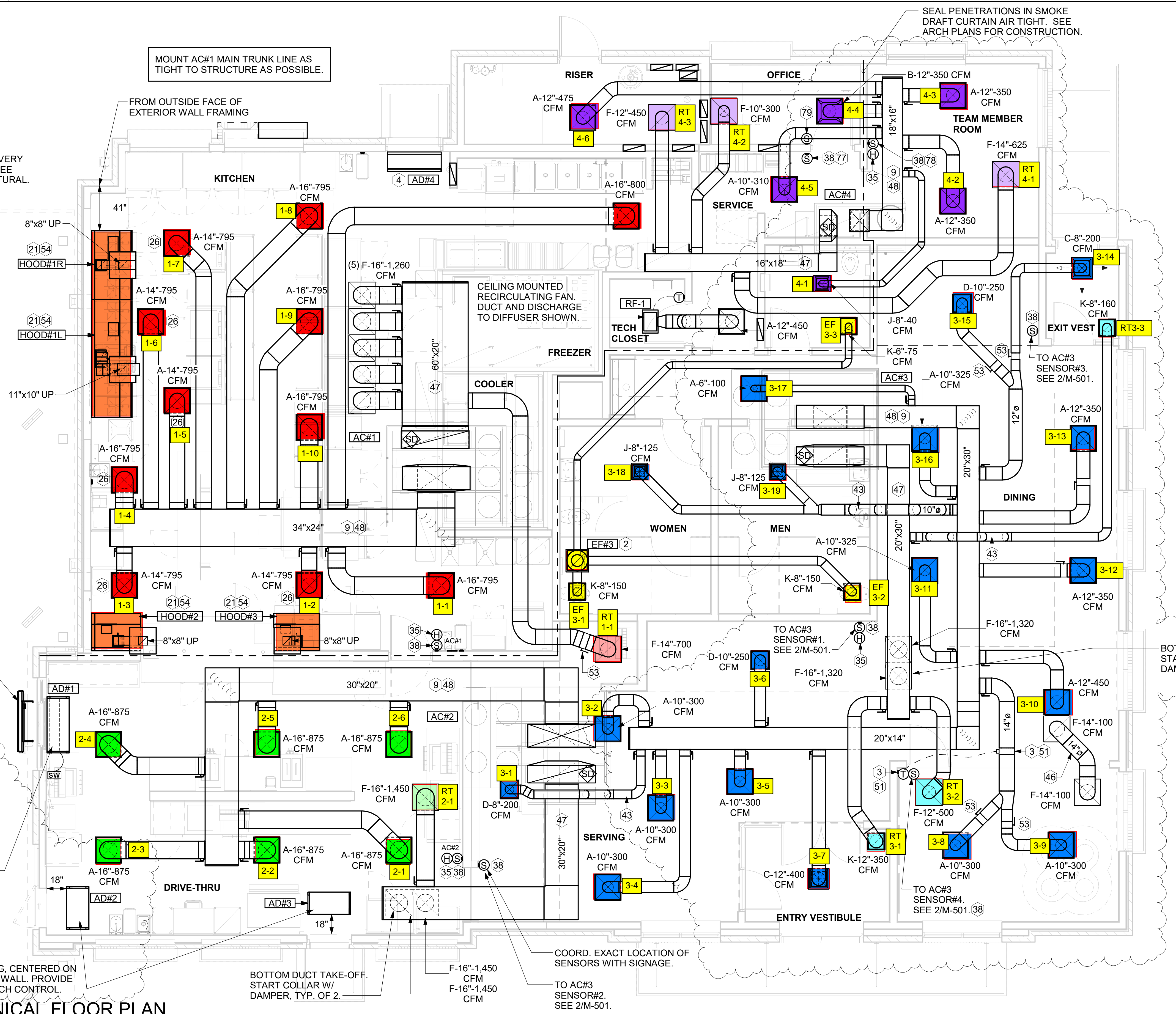
1 MECHANICAL FLOOR PLAN 1/4" = 1'-0"
