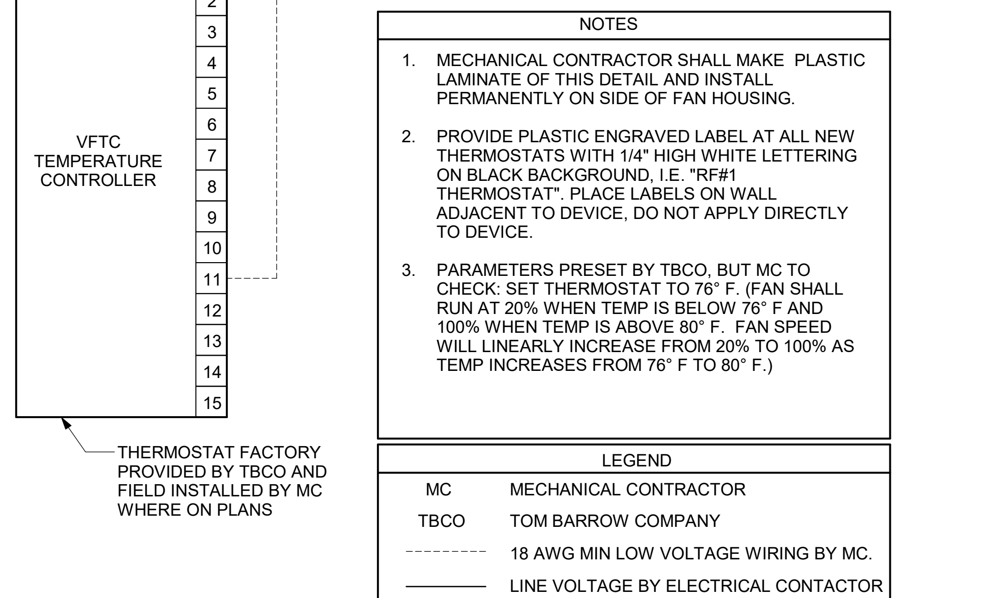
4 TECH CLOSET CONTROL DIAGRAM NOT TO SCALE
