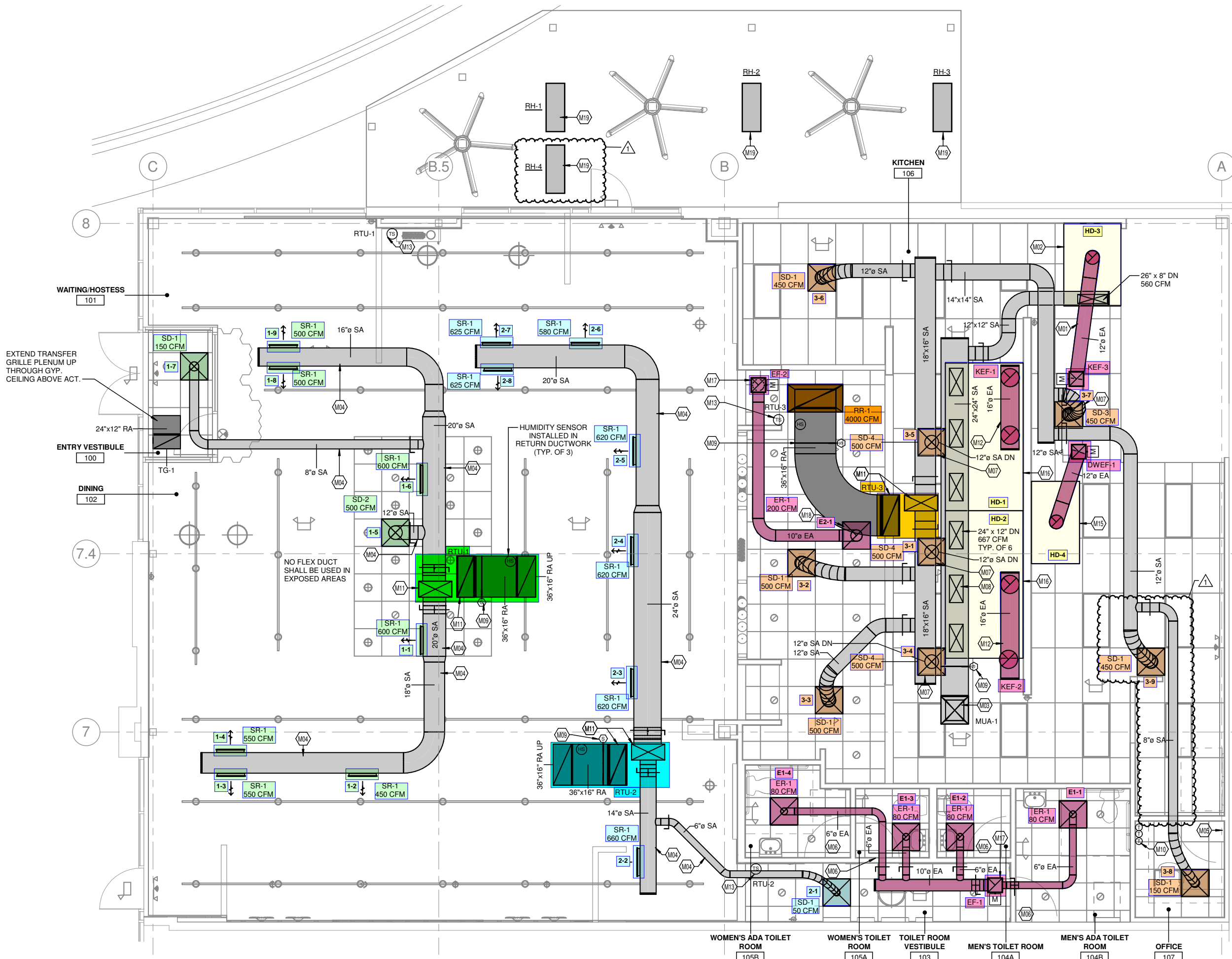
① MECHANICAL FLOOR PLAN
