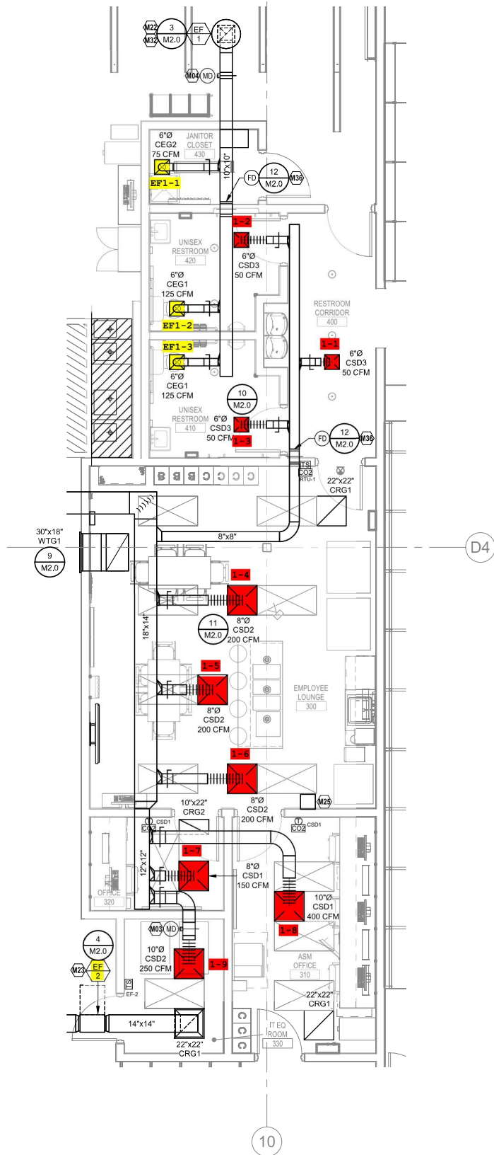
① ENLARGED BACK OF HOUSE HVAC PLAN 1/4" = 1'-0"
