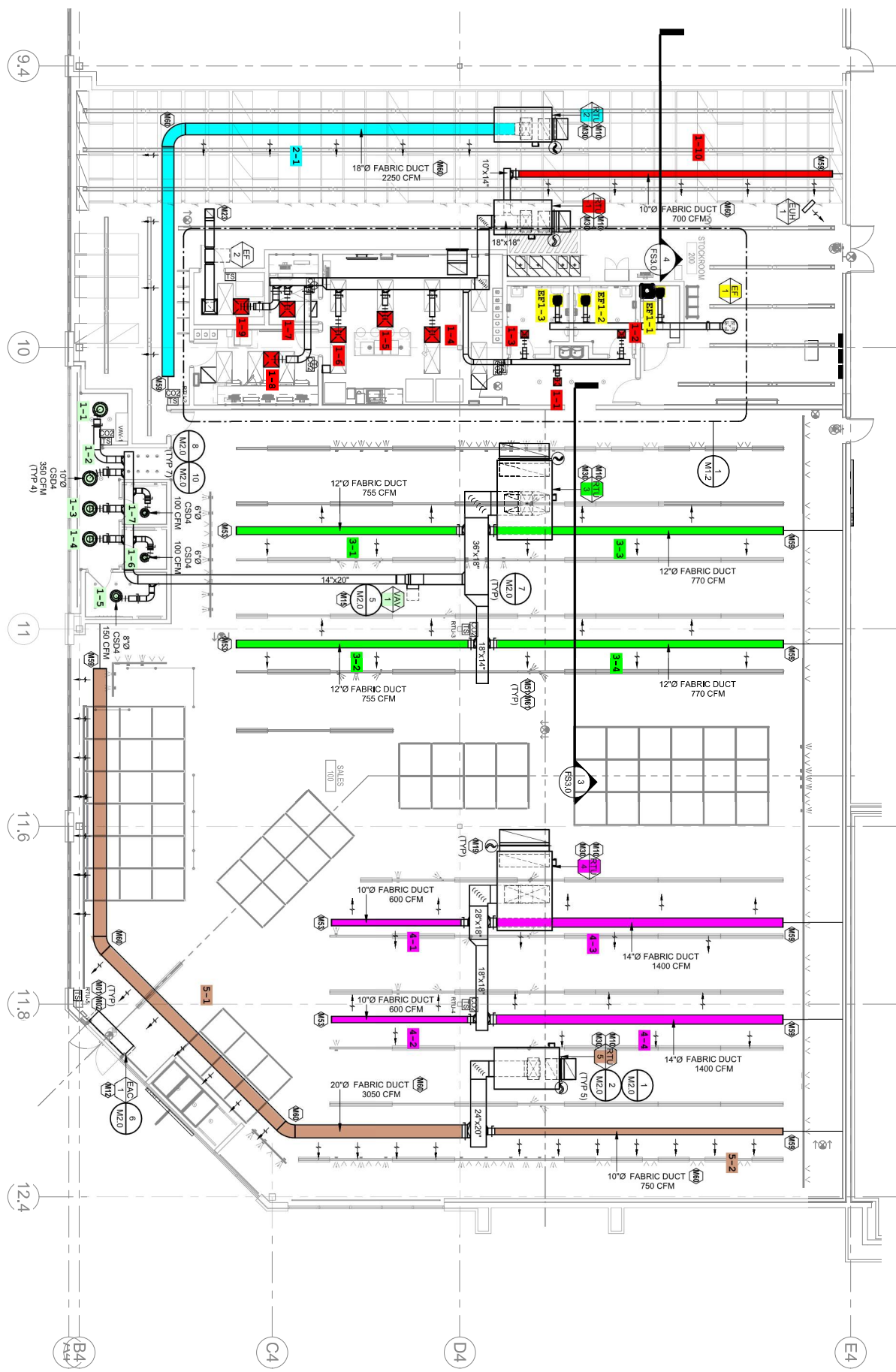
1 HVAC PLAN 1/8" = 1'-0"
