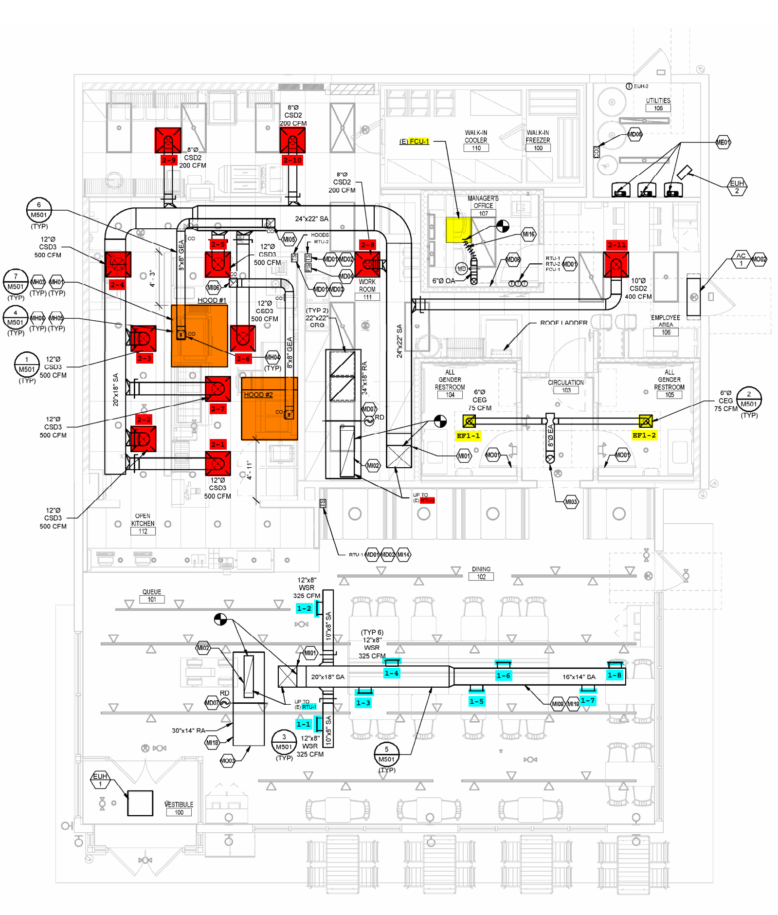
1 MECHANICAL FLOOR PLAN 1/4" = 1'-0"
