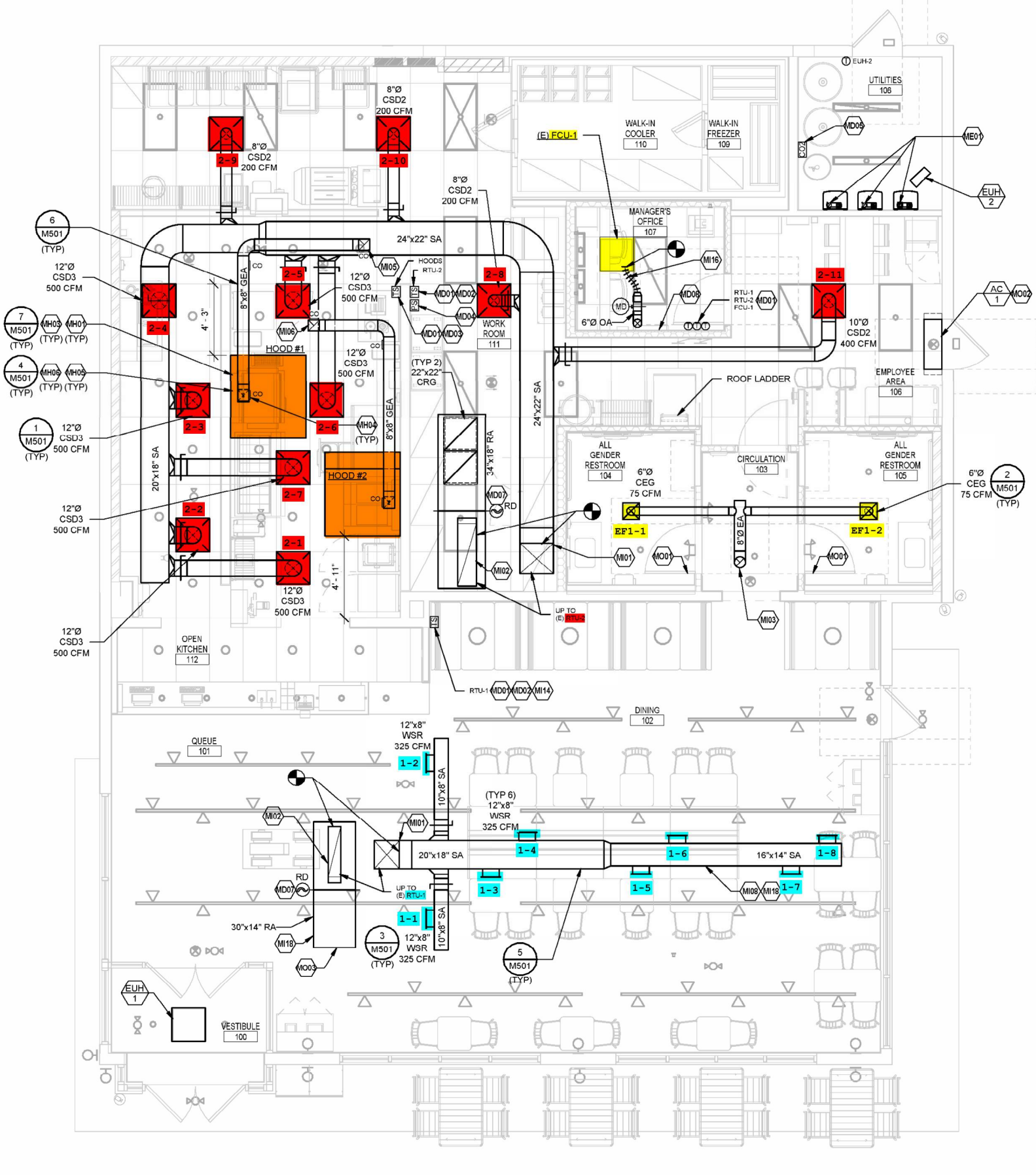
① MECHANICAL FLOOR PLAN 1/4" = 1'-0"
