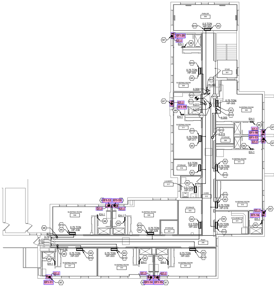
1 3RD FLOOR MECHANICAL PLAN
