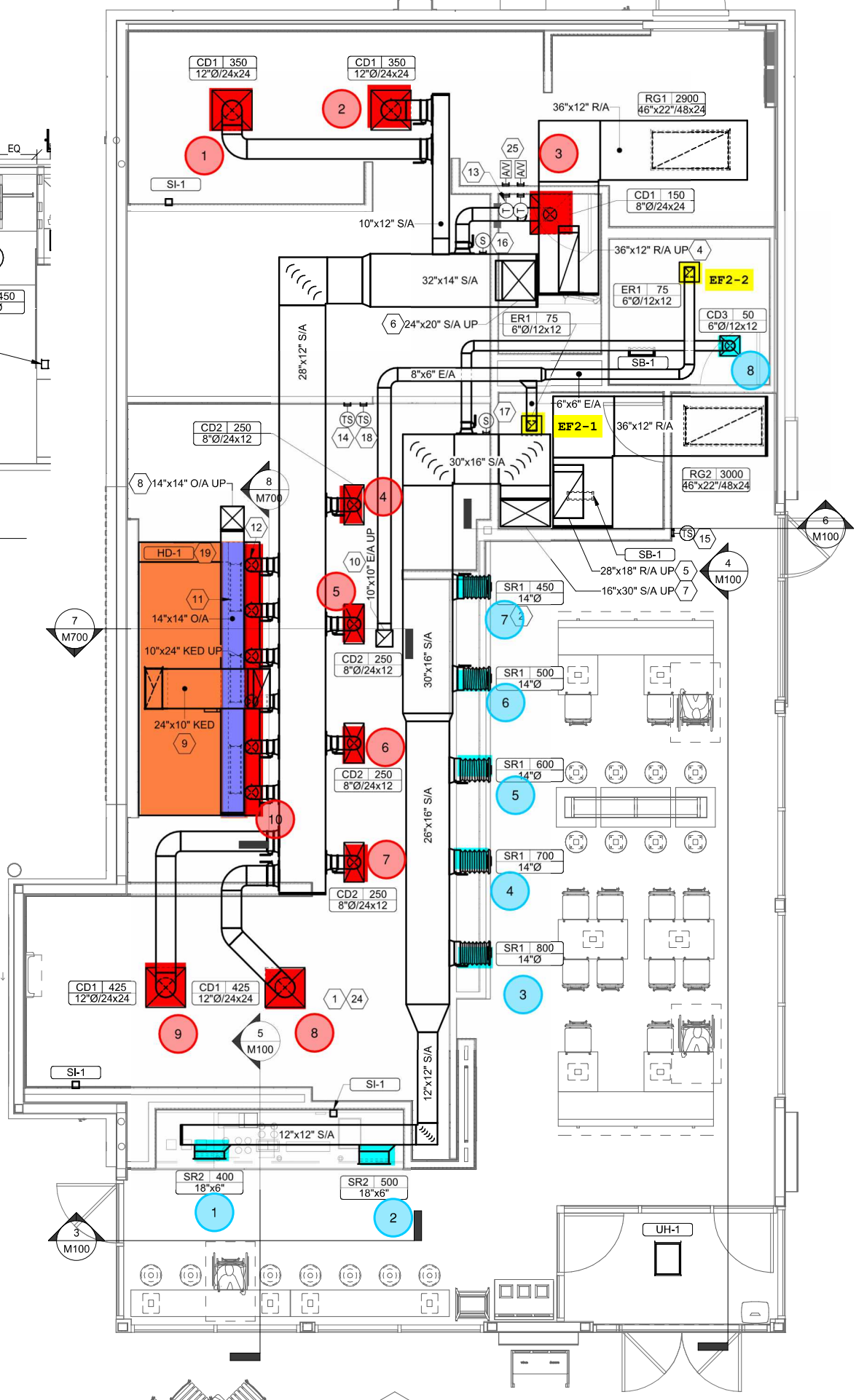
HVAC Floor Plan 1/4" = 1'-0"
