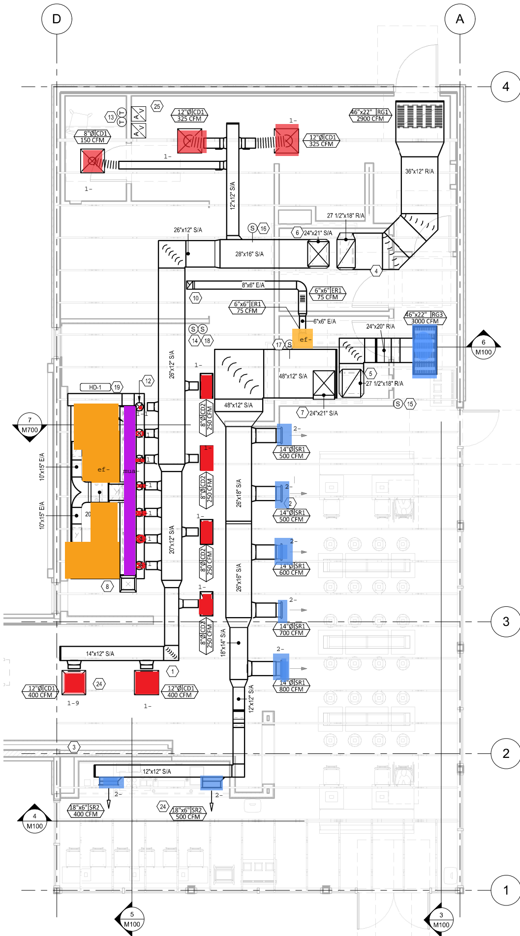
HVAC PLAN 1/4" = 1'-0"
