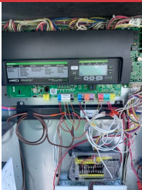
PRODIGY WIRING Typical of 3 RTUs
