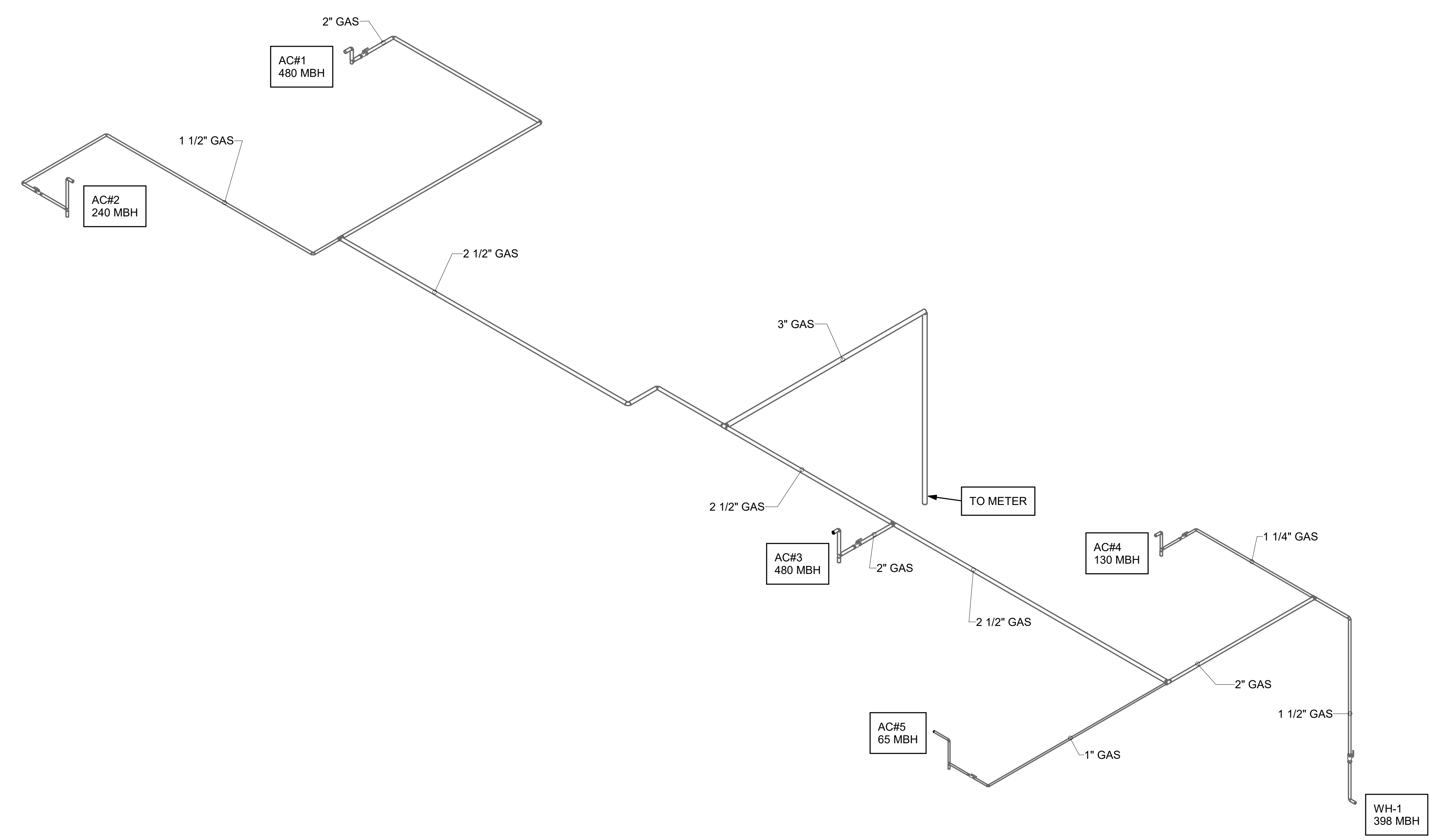
1 GAS PIPING ISOMETRIC - RTUS & WATER HEATER
