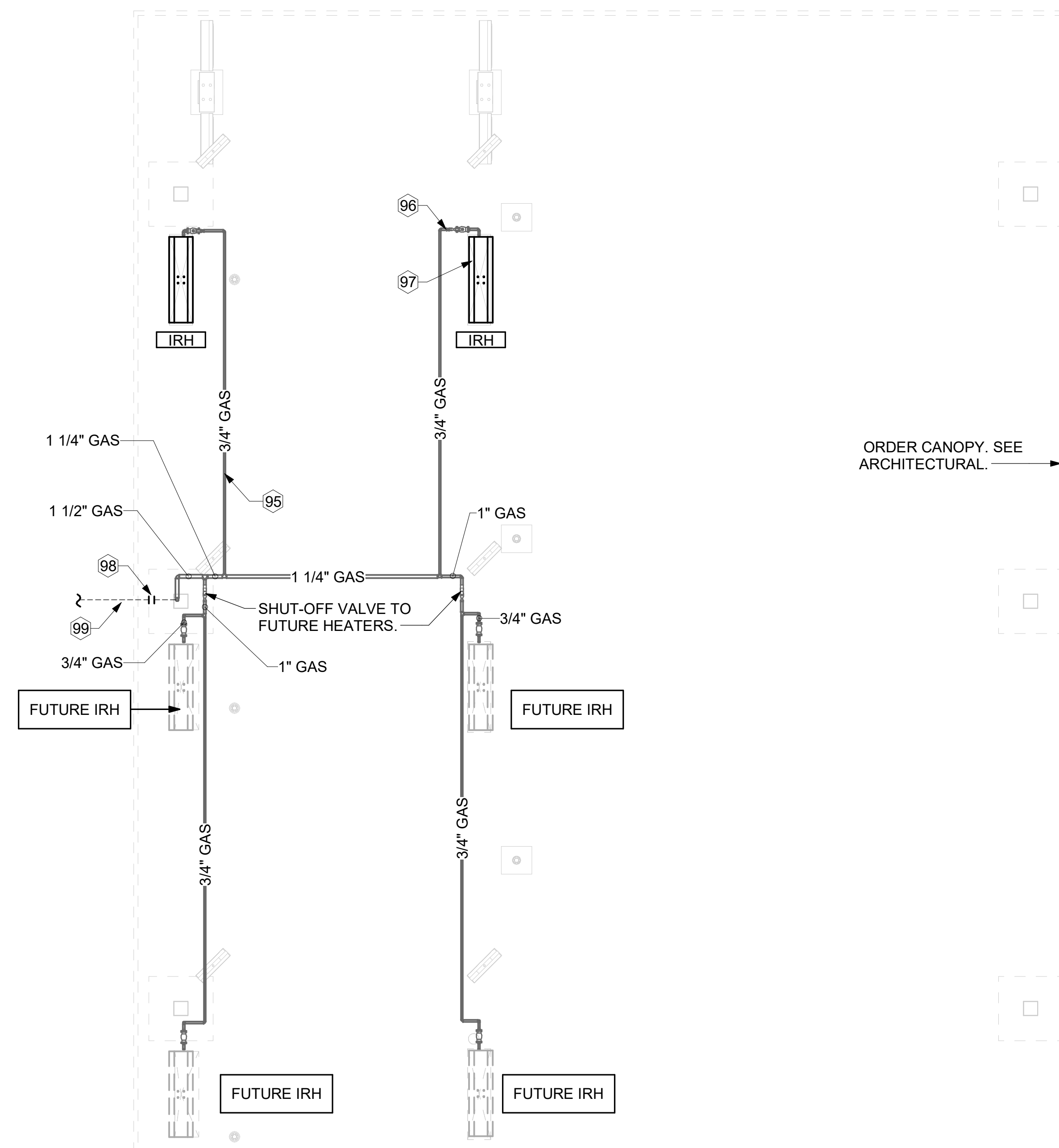
2 ORDER CANOPY GAS PIPING PLAN 1/4" = 1'-0"
