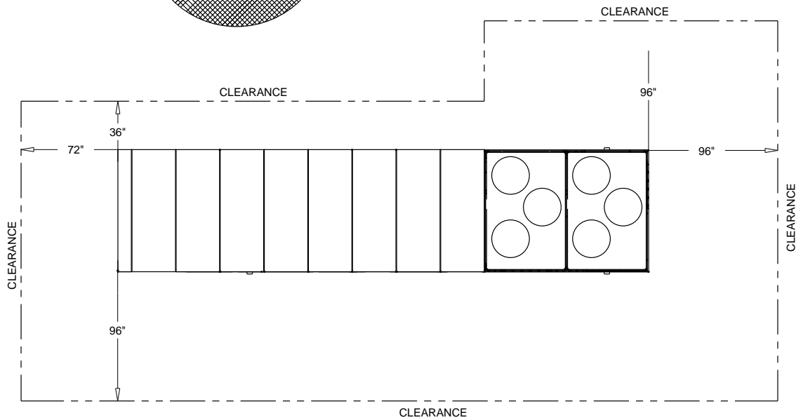
RIGGING AND CLEARANCE AIR COOLED DRAWING
