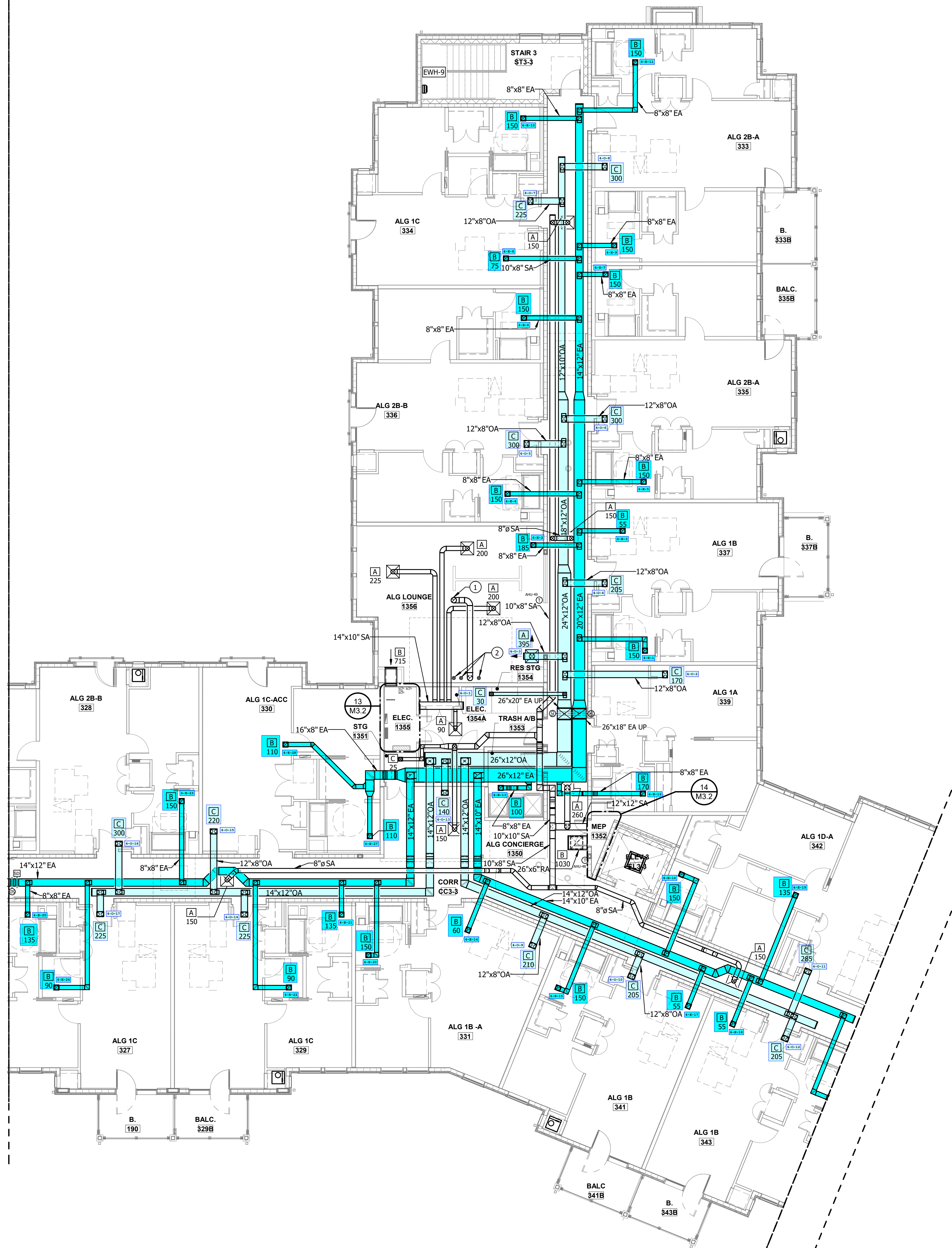
THIRD FLOOR HVAC - WING B SCALE: 1/8" = 1'-0"
