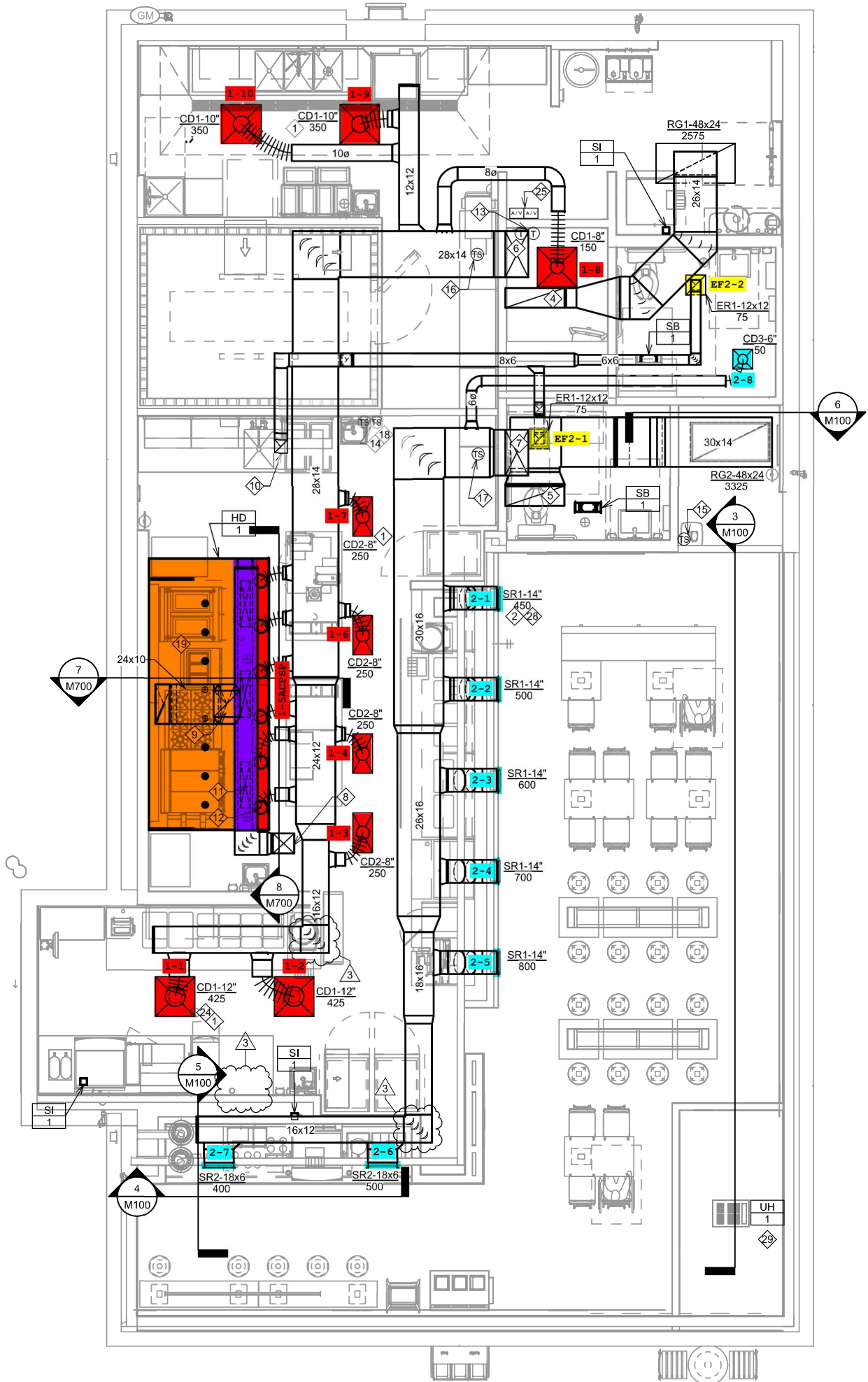
① HVAC FLOOR PLAN 1/4" = 1'-0"
