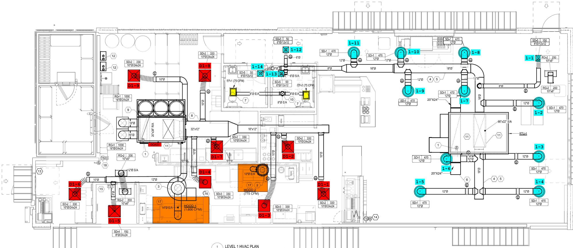
1 LEVEL 1 HVAC PLAN
