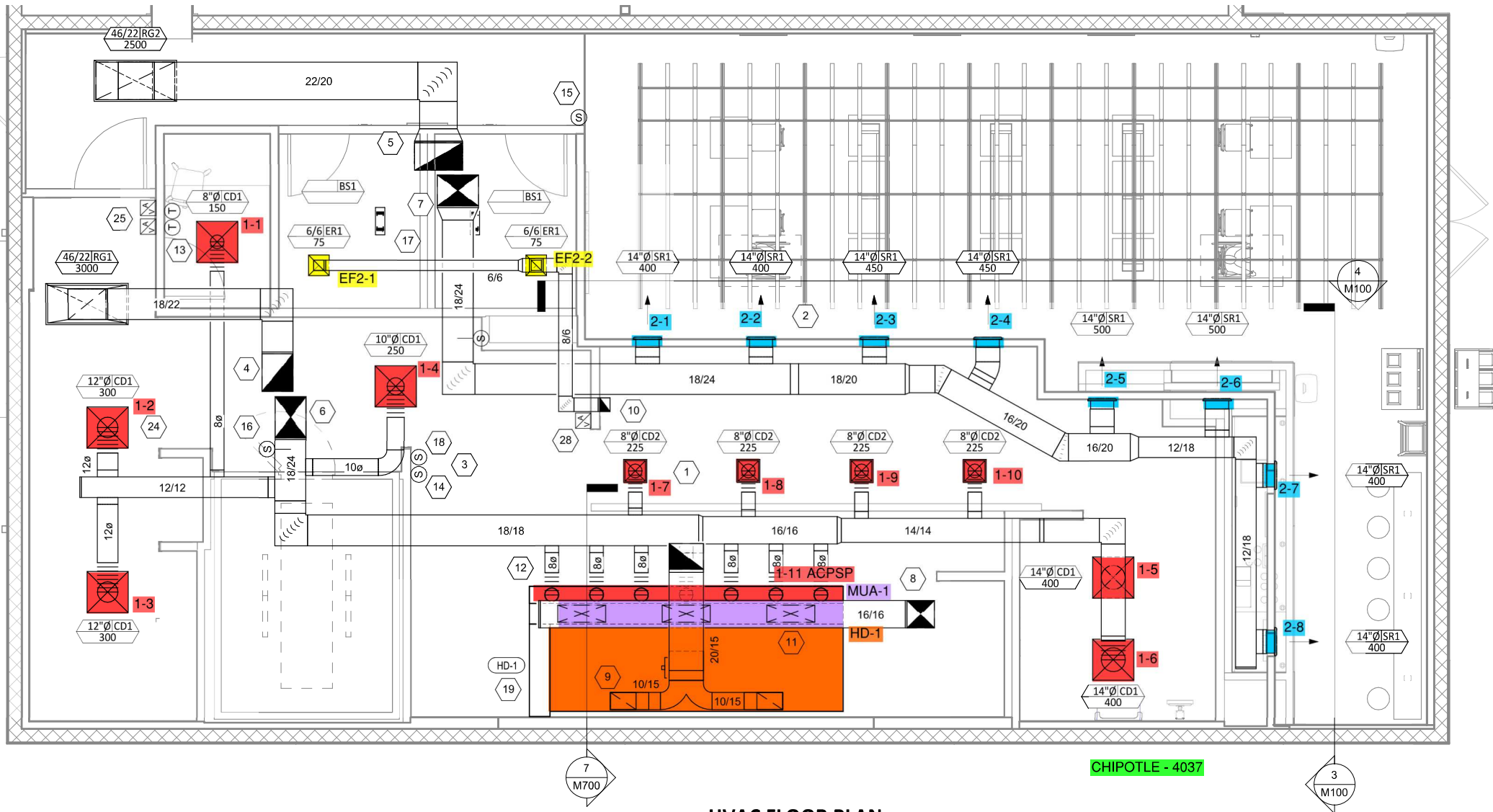
HVAC FLOOR PLAN
